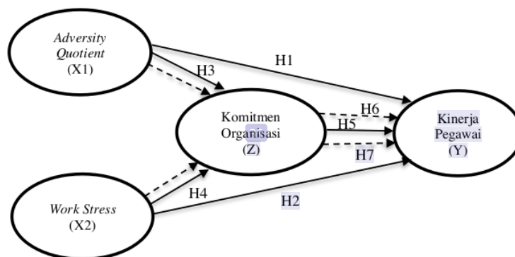
Gambar 1 Model Hipotesis
