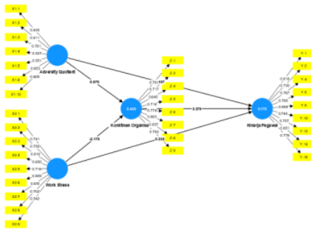
Gambar 2 Outer Model
